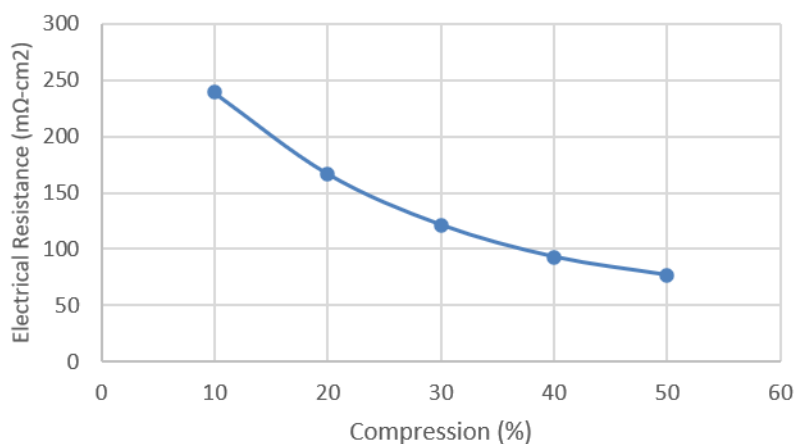
TP Resistance vs. Compression (%)
